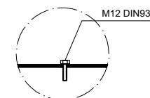
DETAIL M
